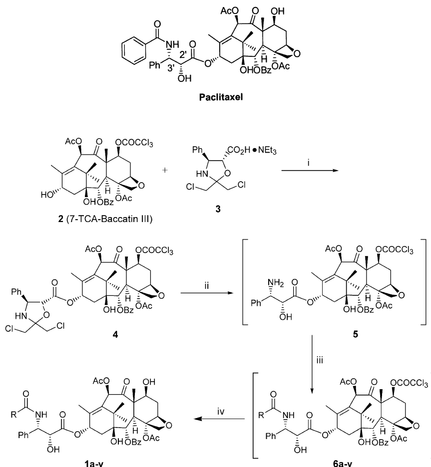
Scheme 1. Reagents and conditions: (i) DCC, toluene, 35 °C, 2 h; (ii) c -HCl, then aq NaHCO 3 , EtOAc; (iii) RCOCl, pyridine; (iv) NH 4 OAc, MeOH–THF.
